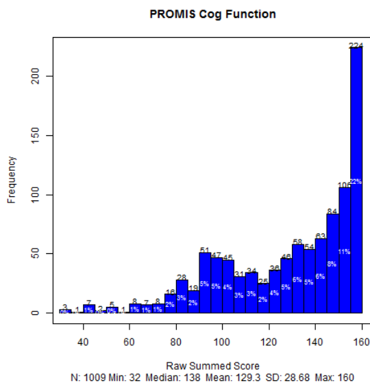
Figure 5.4.1: Raw Summed Score Distribution - PROMIS v2.0 Cognitive Function
