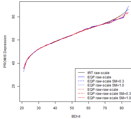
Figure 5.7.10: Equipercentile Linking Functions
