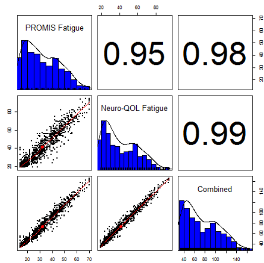
Figure 5.11.4: Scatter Plot Matrix of Raw Summed Scores
