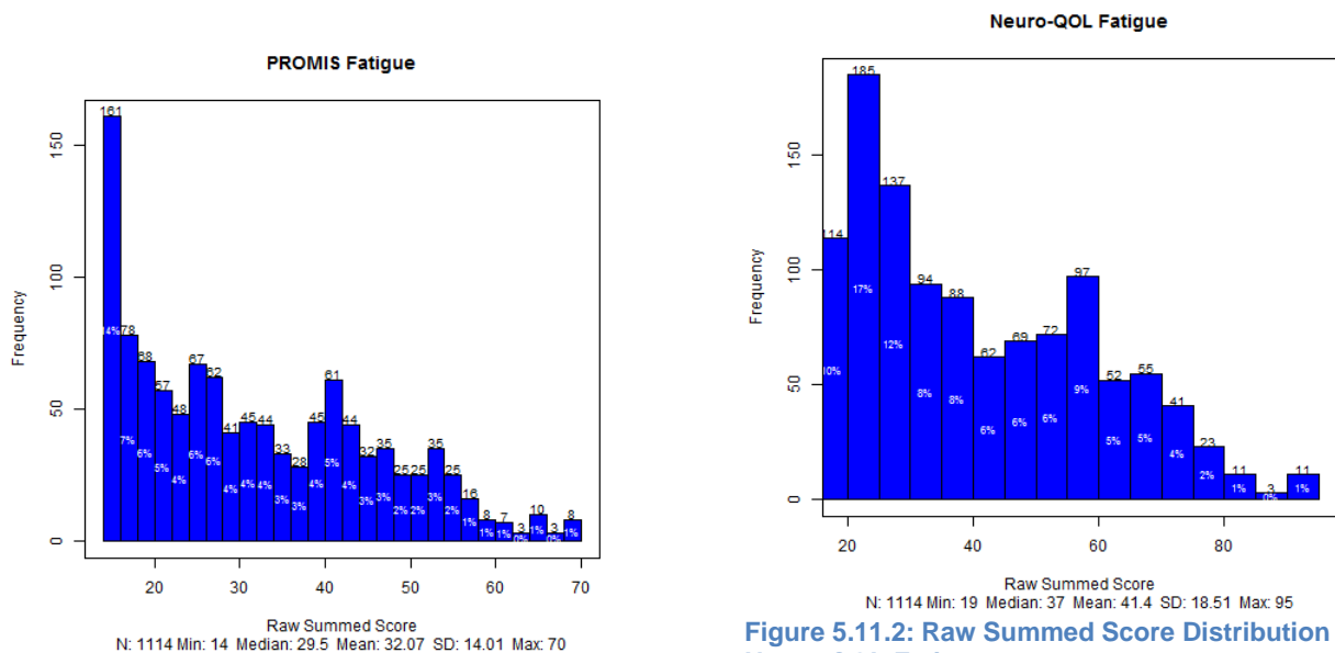
Figure 5.11.1: Raw Summed Score Distribution - PROMIS Fatigue
