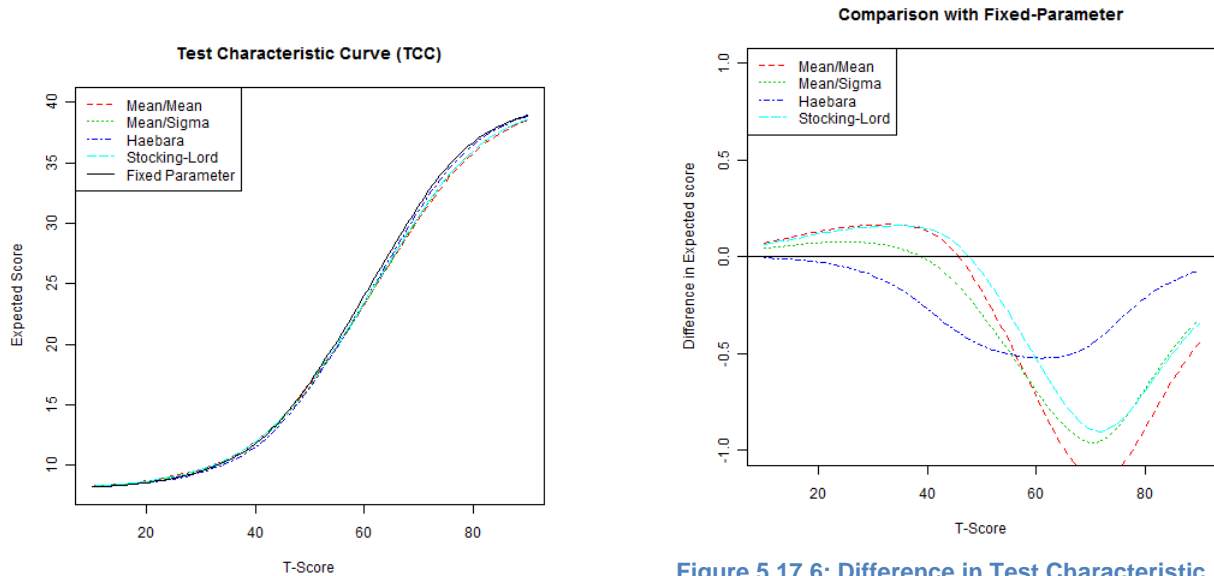
Figure 5.17.5: Test Characteristic Curves (TCC) from Different Linking Methods
