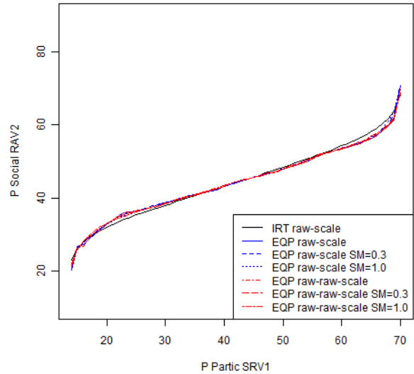
Figure 5.23.10: Equipercentile Linking Functions
