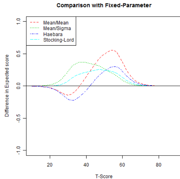
Figure 5.23.6: Difference in Test Characteristic Curves (TCC)
