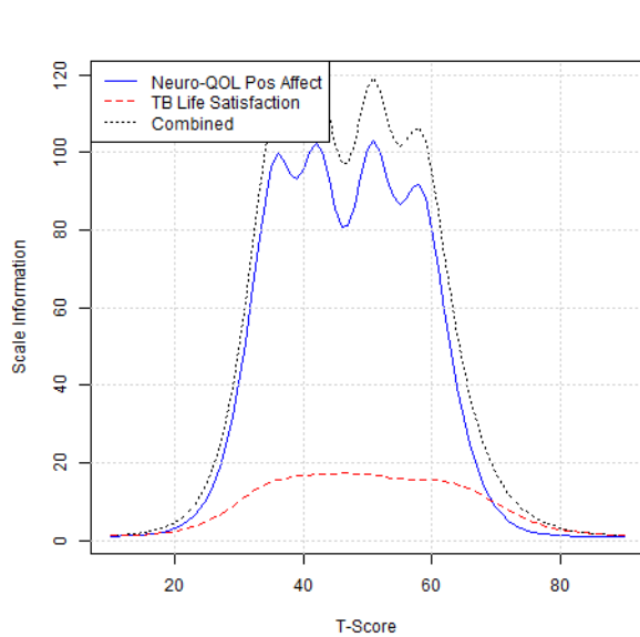
Figure 5.24.7: Comparison of Scale Information Functions
