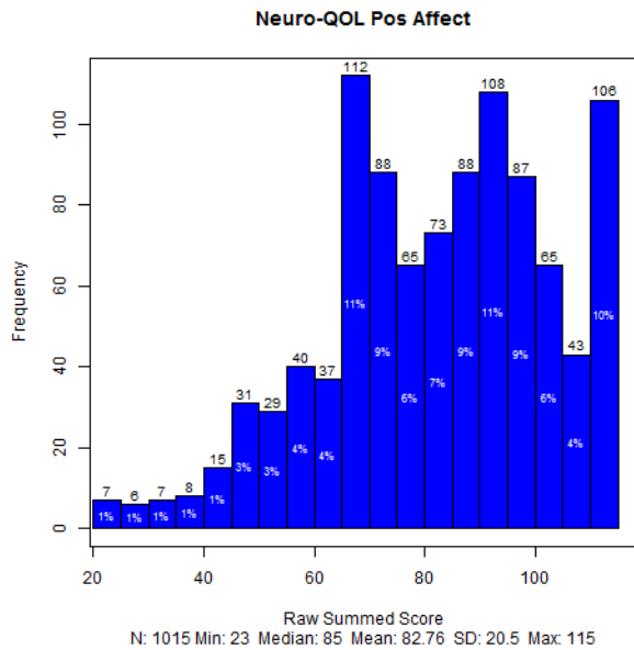
Figure 5.24.1: Raw Summed Score Distribution – Neuro-QoL Positive Affect & Well-being
