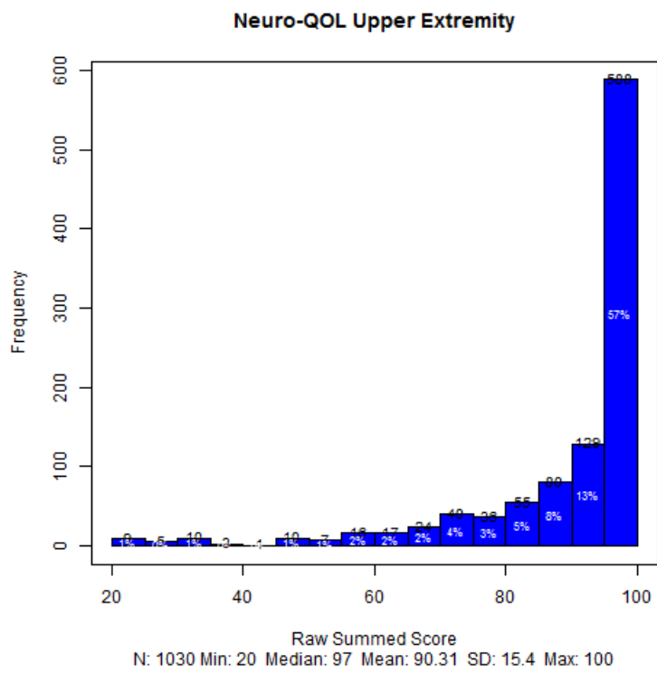
Figure 2: Raw Summed Score Distribution - Neuro-QOL Upper Extremity
