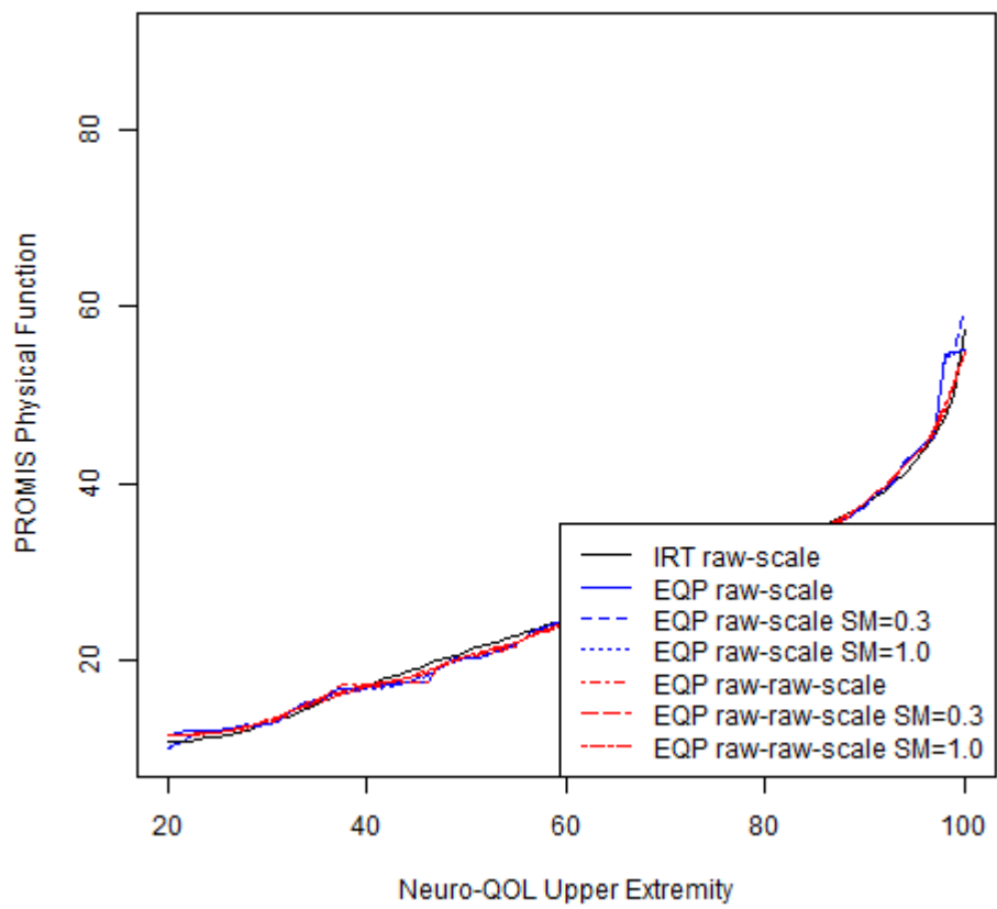
Figure 10: Equipercetile Linking Functions
