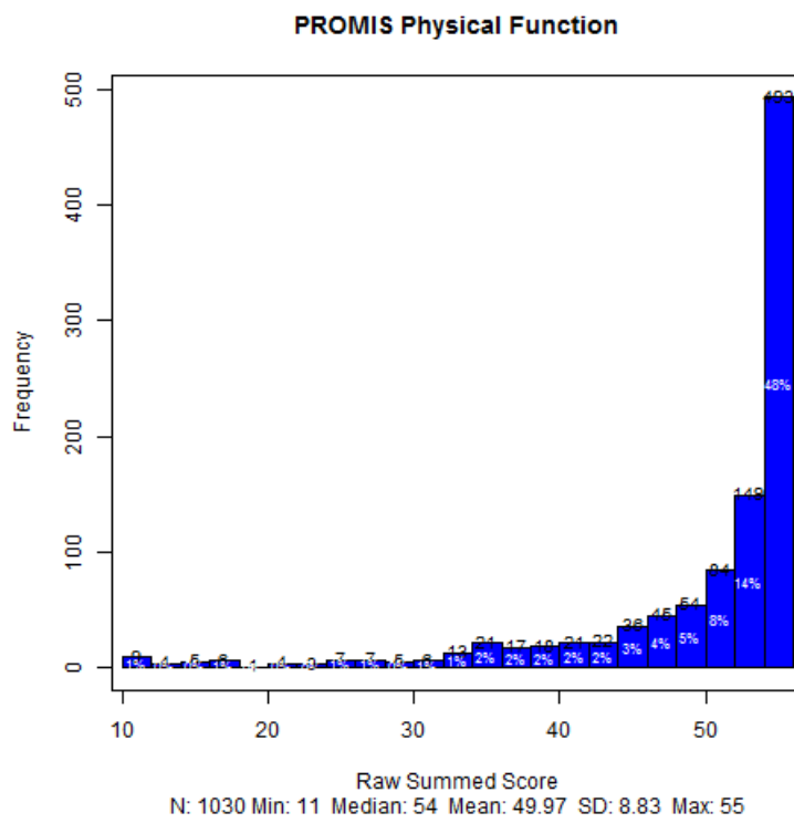
Figure 1: Raw Summed Score Distribution - PROMIS Physical Function
