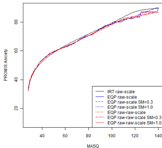
Figure 5.14.10: Equipercntile Linking Functions
