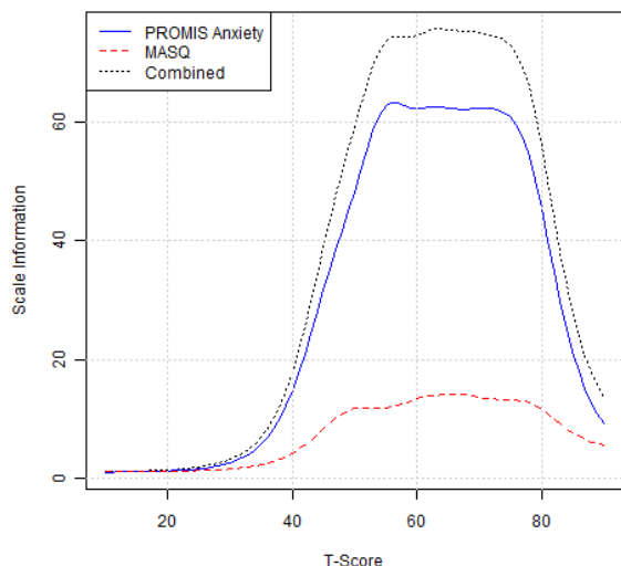
Figure 5.1.7: Comparison of Scale Information Functions
