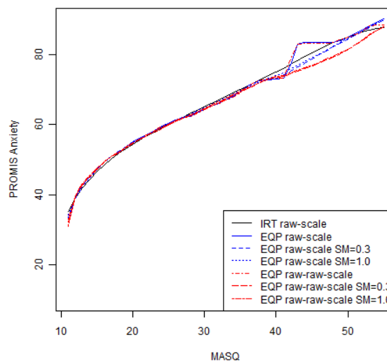
Figure 5.1.10: Equipercentile Linking Functions
