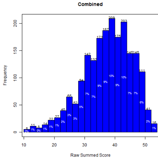
Figure 5.12.3: Raw Summed Score Distribution – Combined
