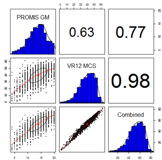
Figure 5.13.2: Scatter Plot Matrix of Raw Summed Scores
