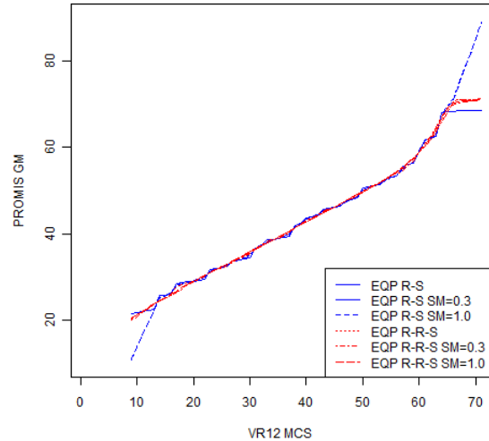
Figure 5.13.4: Equipercentile Linking Functions
