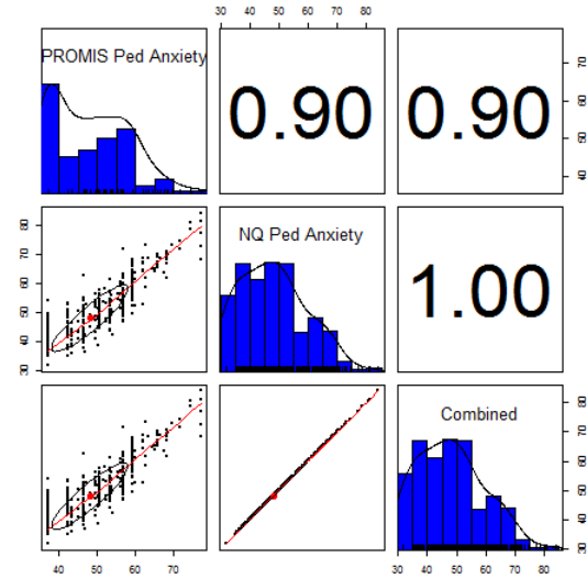
Figure 5.1.10: Comparison of IRT Scaled Scores
