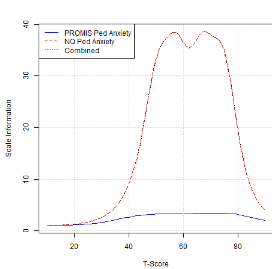
Figure 5.1.9: Comparison of Scale Information Functions
