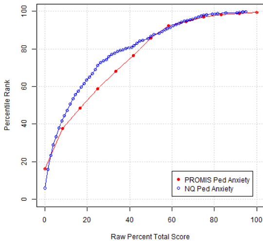
Figure 5.1.11: Comparison of Cumulative Distribution based on Raw Summed Scores
