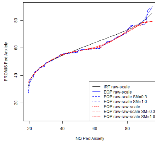
Figure 5.1.12: Equipercentile Linking Functions
