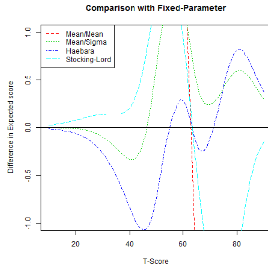
Figure 5.3.6: Difference in Test Characteristic Curves (TCC) from Different Linking Methods
