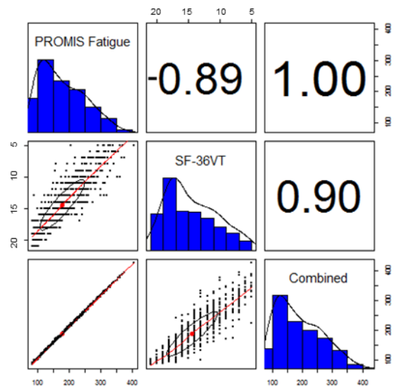
Figure 5.9.4: Scatter Plot Matrix of Raw Summed Scores
