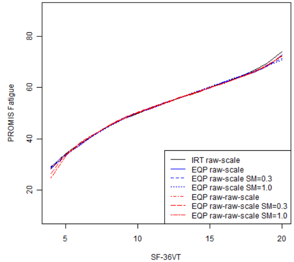
Figure 5.9.10: Equipercentile Linking Functions
