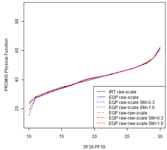
Figure 5.7.10: Equipercntile Linking Functions
