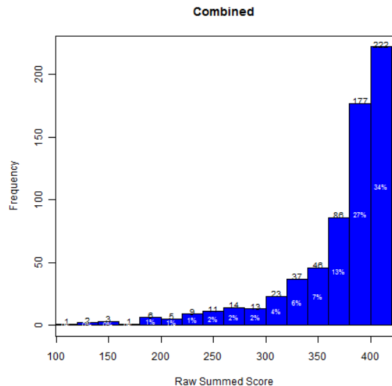
Figure 5.7.3: Raw Summed Score Distribution – Combined
